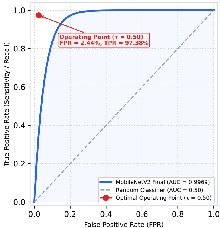
Figure 4(b): Receiver Operating Characteristic (ROC) (Confirming Near-Perfect Class Discrimination)
