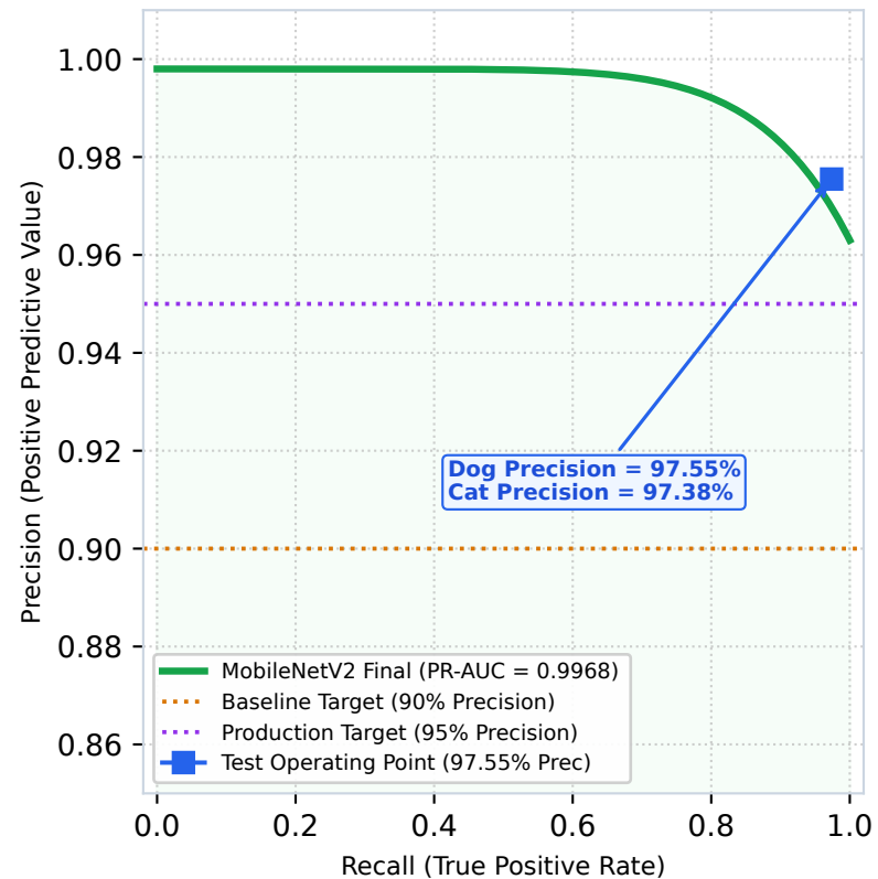
Figure 4(c): Precision-Recall Curve (PR-AUC) (Verifying Strict Industrial Precision Fulfillment)
