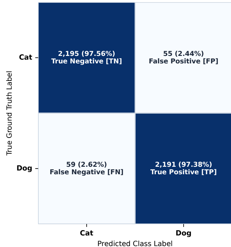
Figure 4(a): Normalized Confusion Matrix (Holdout Test Set, N = 4,500 Images)
